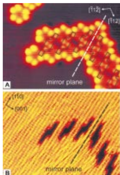
Figure 2. A) Constant current images ( 110 \times 82 \text{ \AA}^2 ) of the HtBDC double-row structure and immobilized single molecules at 25 K ( V = 1250 \text{ mV} , I = 0.42 \text{ nA} ). Holes in the restructured surface are framed black. B) Holes underneath the molecules after pushing the molecules aside. The holes consist of approximately 14 Cu atoms expelled from the surface in two adjacent [1\bar{1}0] rows ( V = 10 \text{ mV} , I = 1.78 \text{ nA} ).
