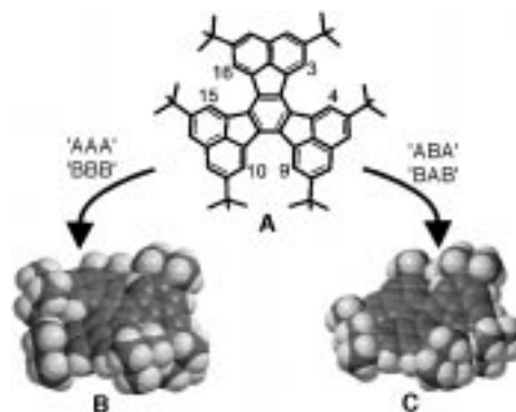
Figure 1. A) Molecular structure of 2,5,8,11,14,17-hexa-( tert -butyl)decacyclene (HtBDC). Space-filling model of the two low-energy conformations: B) propeller shape of the AAA/BBB conformation, and C) boat shape of the ABA/BAB conformation. [19] The numbers label the positions of the interacting hydrogen atoms that lead to the local A and B conformations (see text for details).
